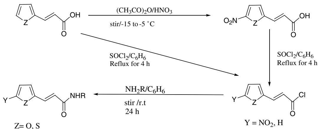
Scheme 1. General procedure for the chemical synthesis of the eight compounds.
